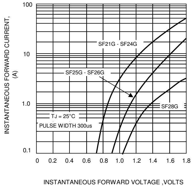
FIG.4-TYPICAL FORWARD CHARACTERISTICS
