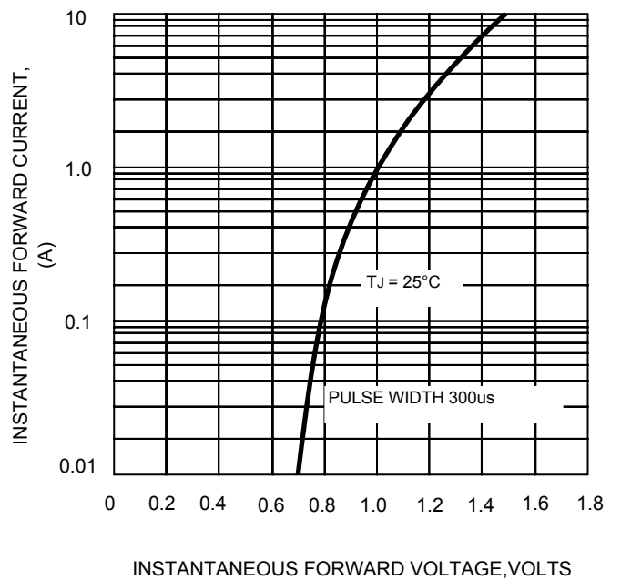
FIG.4-TYPICAL FORWARD CHARACTERISTICS
