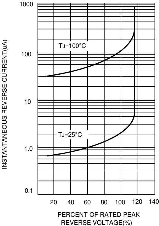
FIG.2-TYPICAL REVERSE CHARACTERISTICS
