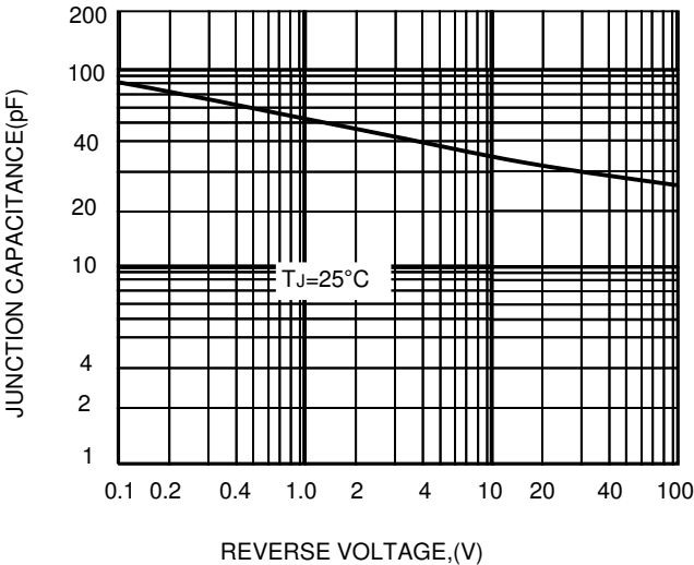
FIG.5-TYPICAL JUNCTION CAPACITANCE
