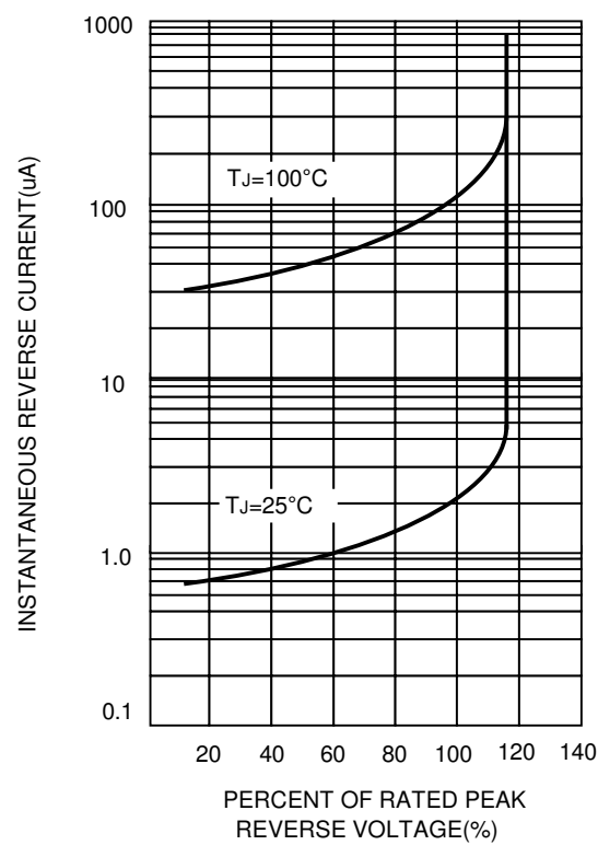
FIG.2-TYPICAL REVERSE CHARACTERISTICS
