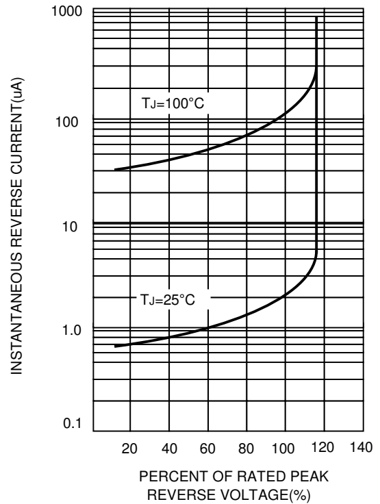
FIG.2-TYPICAL REVERSE CHARACTERISTICS
