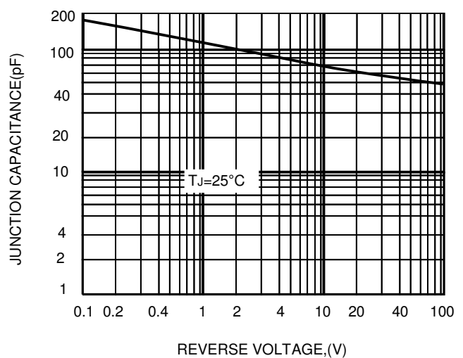
FIG.5-TYPICAL JUNCTION CAPACITANCE
