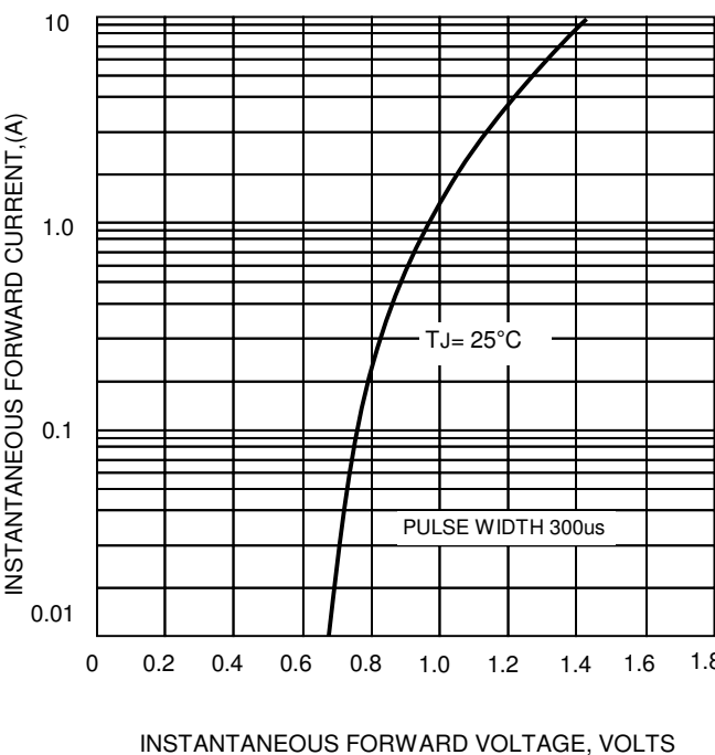
FIG.4-TYPICAL FORWARD CHARACTERISTICS
