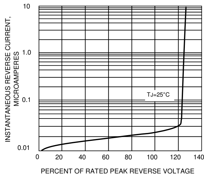
FIG.3-TYPICAL REVERSE CHARACTERISTICS
