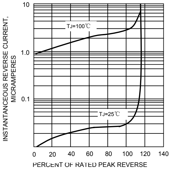
FIG.4-TYPICAL REVERSE CHARACTERISTICS
