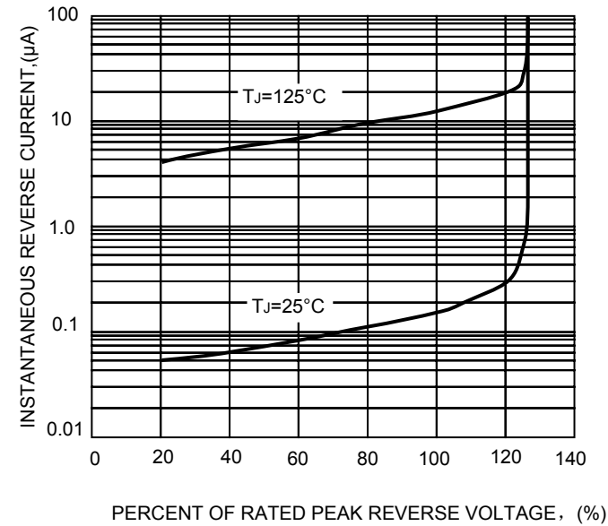
FIG.3-TYPICAL REVERSE CHARACTERISTICS
