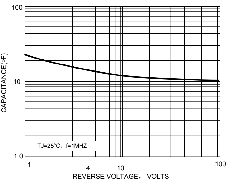
FIG.5-TYPICAL JUNCTION CAPACITANCE
