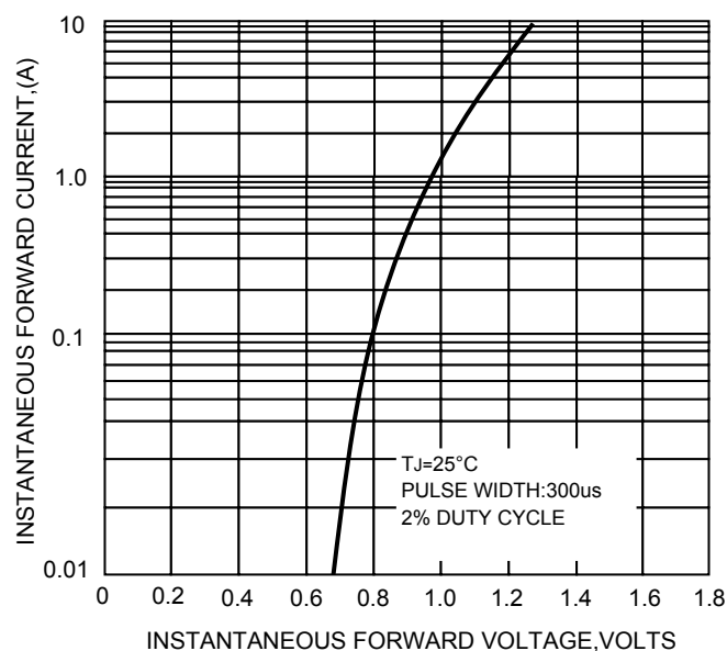
FIG.4-TYPICAL FORWARD CHARACTERISTICS
