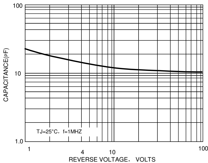
FIG.5-TYPICAL JUNCTION CAPACITANCE
