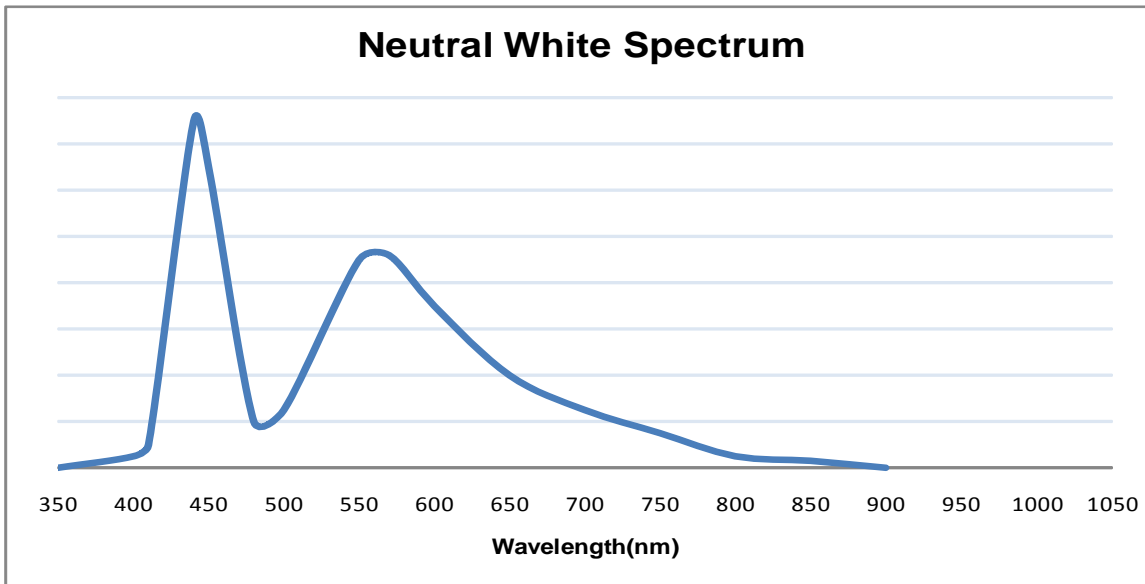
<Figure 3 neutral white color spectrum of HT71 typical CCT part, integrated measurement>
