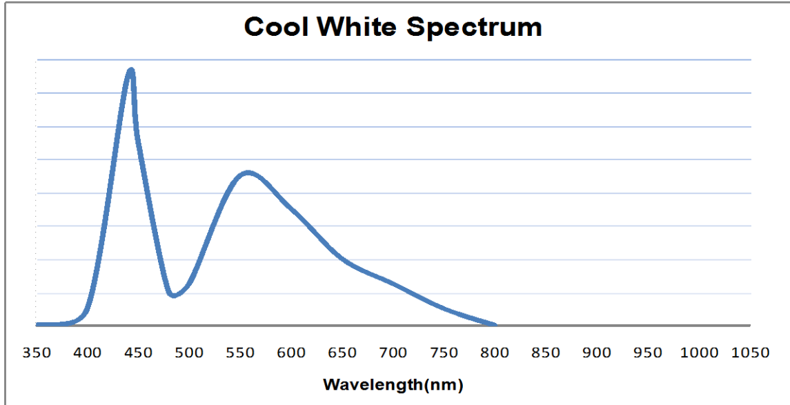
<Figure 2 cool white color spectrum of HT71 typical CCT part, integrated measurement>
