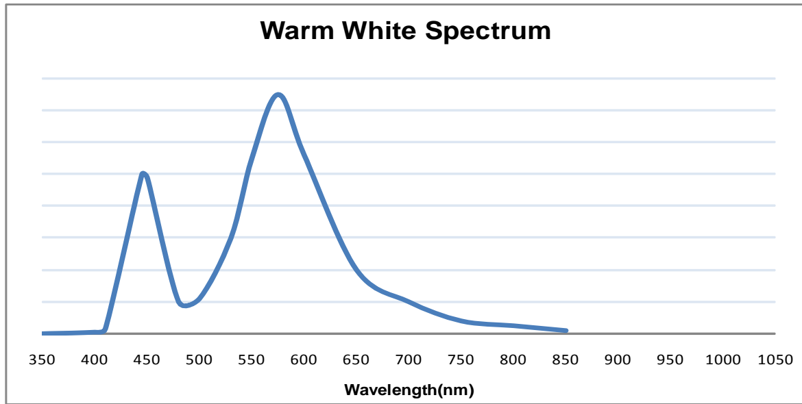
<Figure 4 warm white color spectrum of HT71 typical CCT part, integrated measurement>
