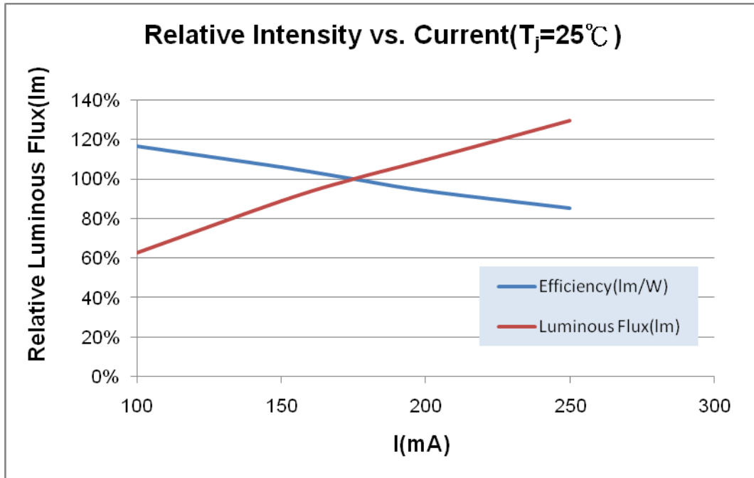
<Figure 2 The trend chart for relative intensity vs. current of HT71C, HT71W>
