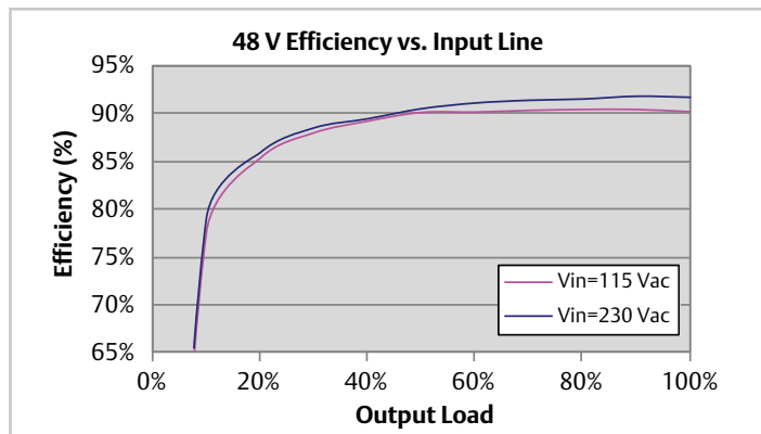
Fig 12. 48 V Efficiency Curve
