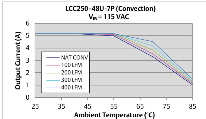
Fig 10. 48 V “7P” Suffix (Convection) Output Current Derating at 115 Vac
