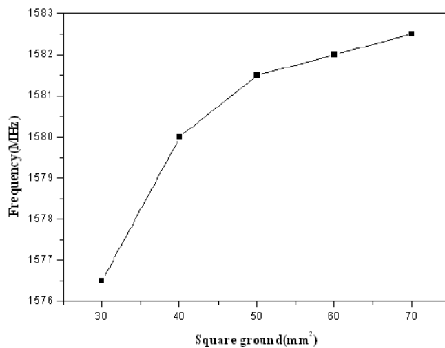
Fig. 6 Center Frequency V.S. Ground Plane
