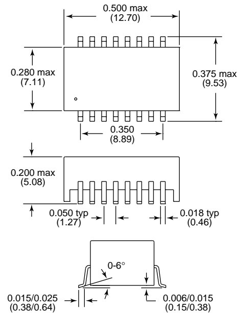
N Package
