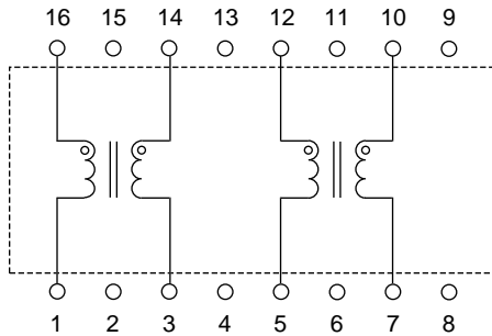
LG01 Circuit
