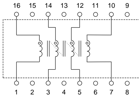
LG11 Circuit
