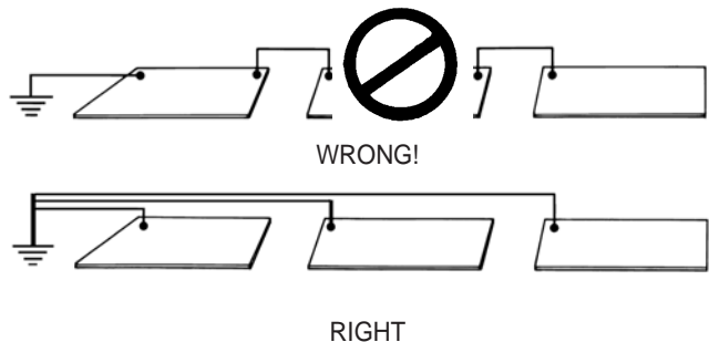
Figure 4. ESD mats should never be grounded in series, that is daisy chained.
