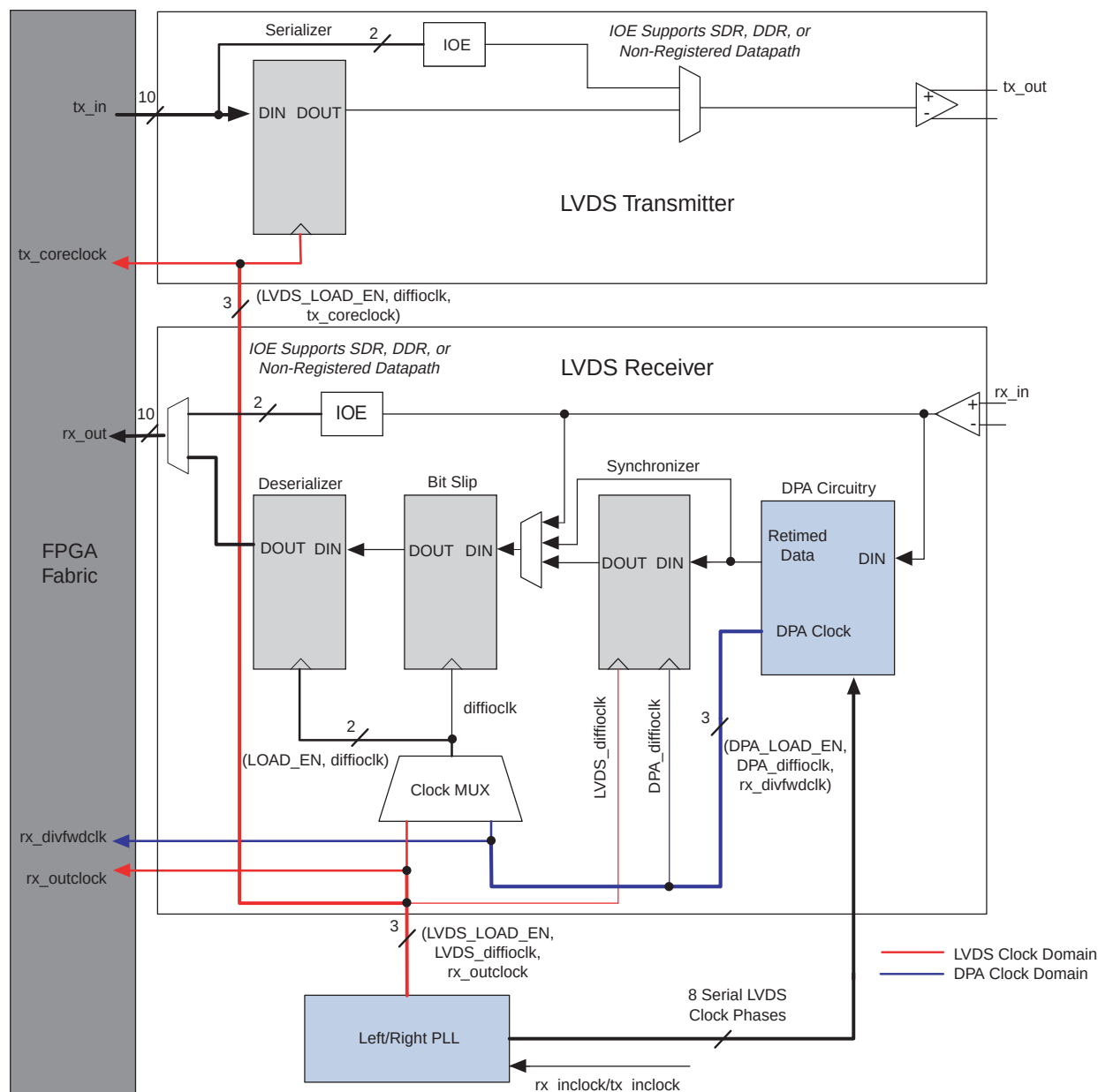
Figure 8-4. LVDS SERDES (1), (2), (3)
