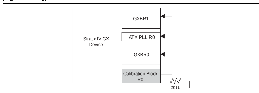
Figure 1-171. Calibration Block Locations in Stratix IV GX Devices with Two Transceiver Blocks (Right Side Only)
