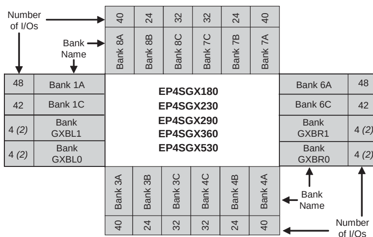
Figure 6–11. Number of I/Os in Each Bank in EP4SGX180, EP4SGX230, EP4SGX290, EP4SGX360, and EP4SGX530 Devices in the 1152-Pin FineLine BGA Package (1) , (2)
