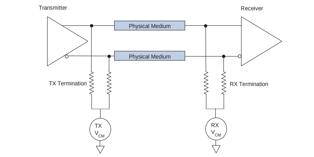
Figure 1-34. DC-Coupled Link
