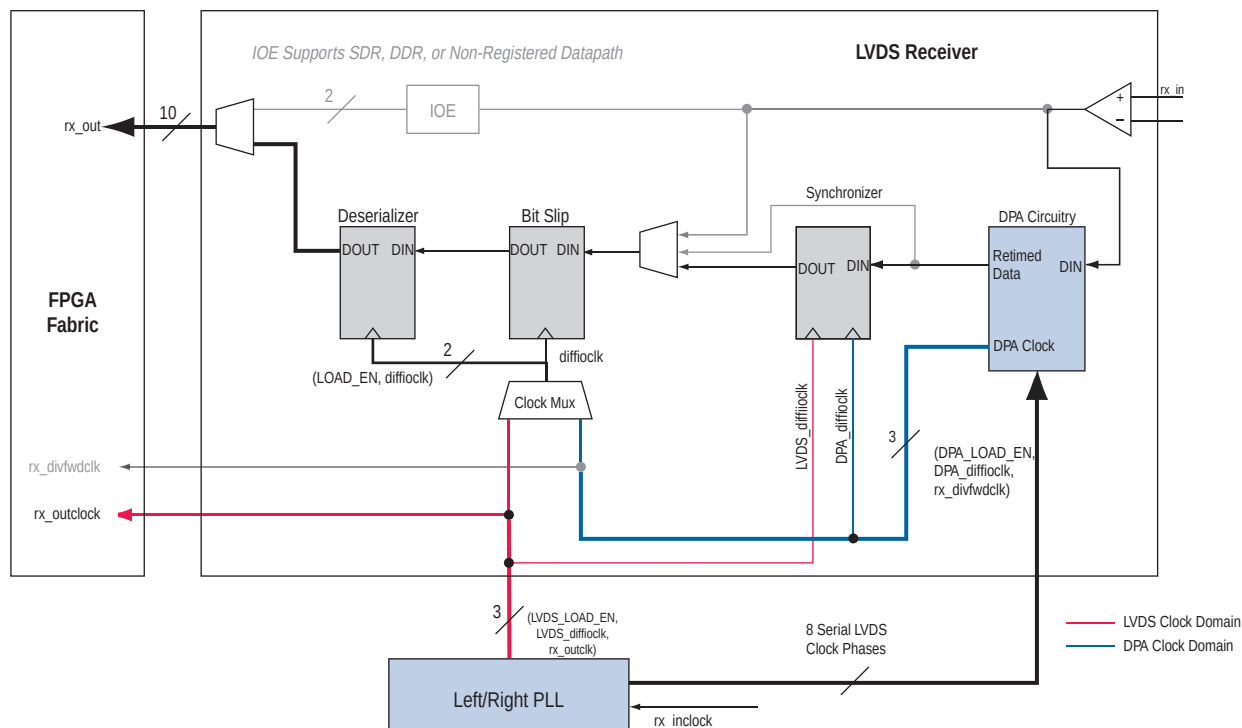
Figure 8-19. Receiver Datapath in DPA Mode (1), (2), (3)
