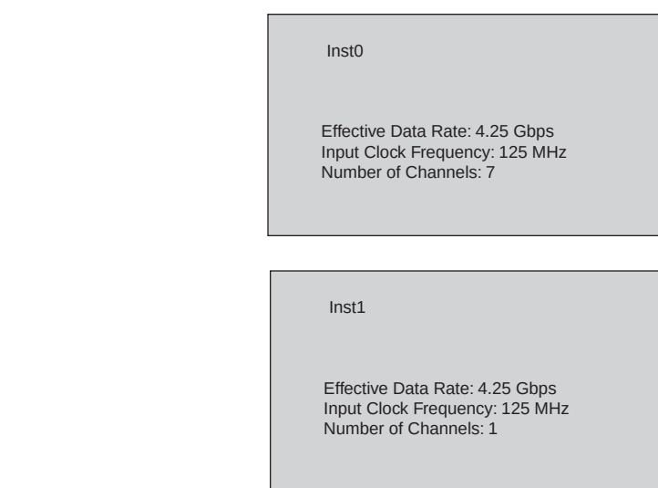
Figure 3-5. Transceiver Channel Instances Before Compilation for Example 4
