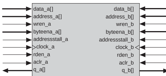
Figure 3-12. Stratix IV True Dual-Port Memory (1)
