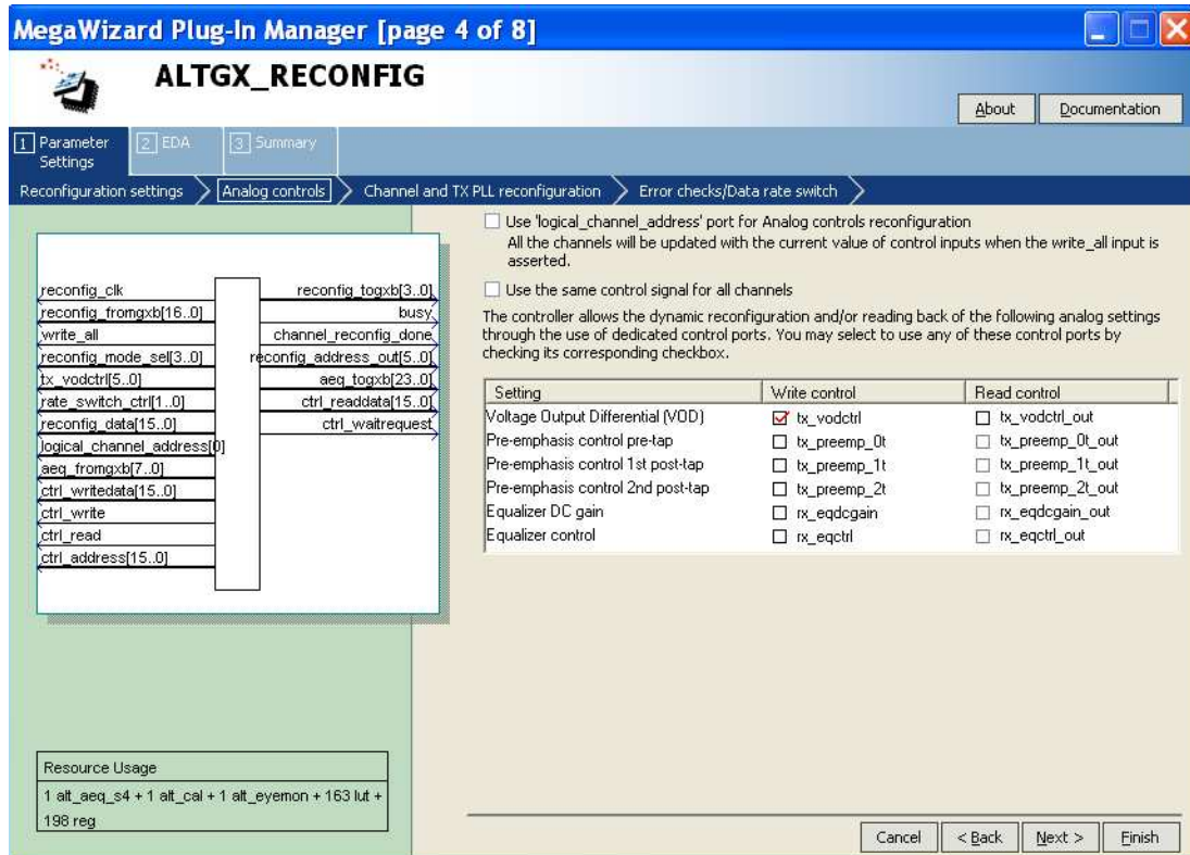
Figure 3-4. MegaWizard Plug-In Manager—ALTGX_RECONFIG (Analog Controls)
