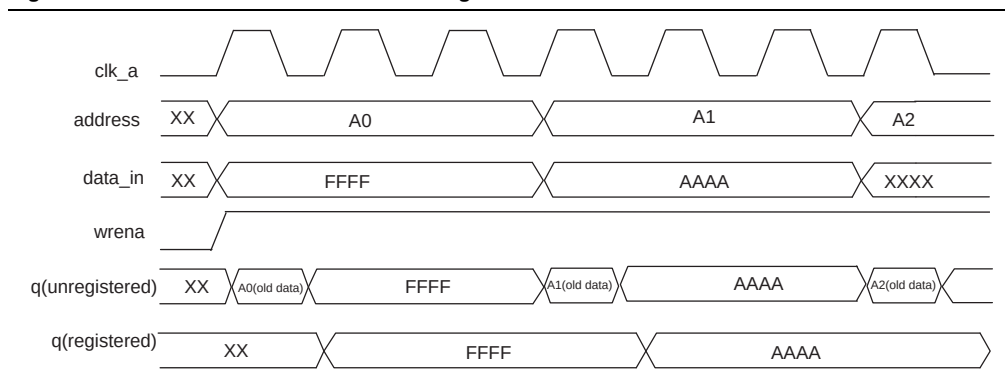
Figure 3-16. MLABs Same-Port Read-During Write: Don't Care Mode
