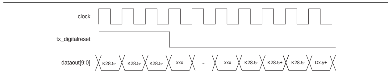
Figure 1–20. 8B/10B Encoder Output During \text{tx\_digitalreset} Assertion
