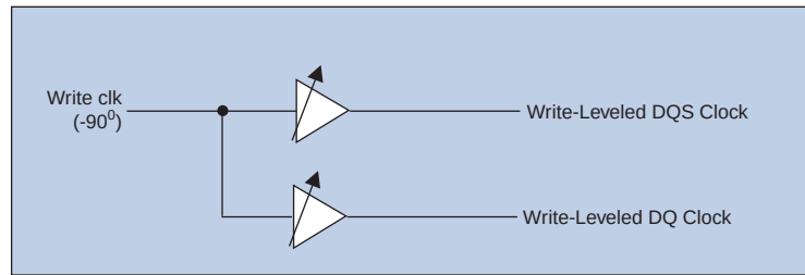
(1) There is one leveling delay chain per I/O sub-bank (for example, I/O sub-banks 1A, 1B, and 1C). You can only have one memory interface in each I/O sub-bank when you use the leveling delay chain.
