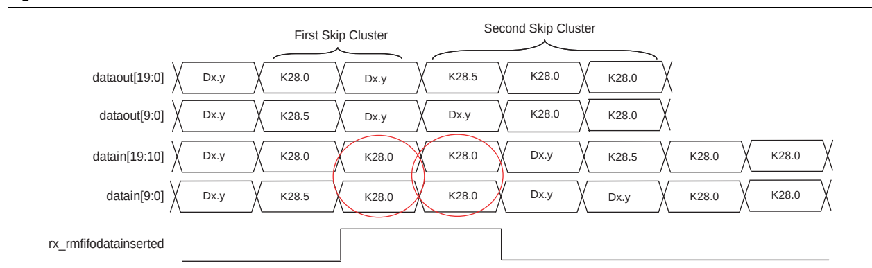
Figure 1-73. Rate Match Insertion in Basic Double-Width Mode
