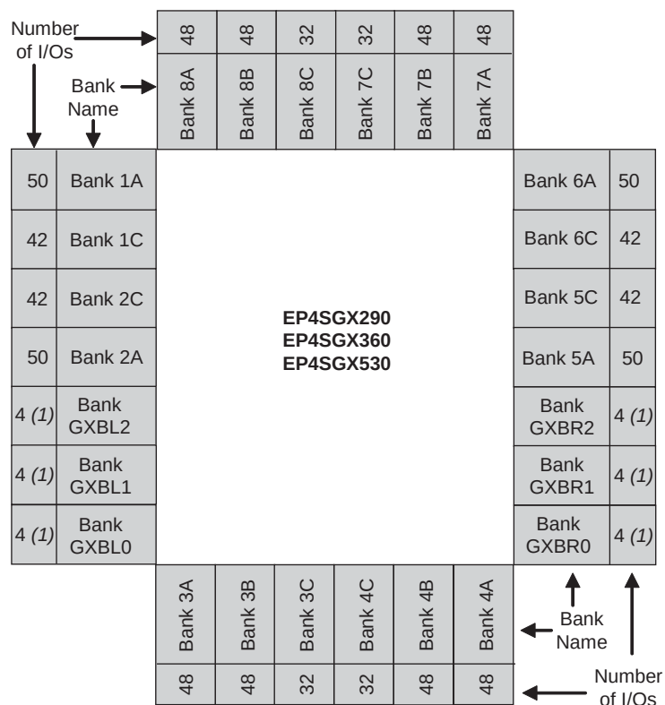
Figure 6-14. Number of I/Os in Each Bank in EP4SGX290, EP4SGX360, and EP4SGX530 Devices in the 1760-Pin FineLine BGA Package (1)
