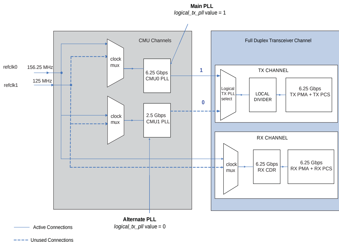
Figure 5-15. Reconfiguring the CMU0 PLL
