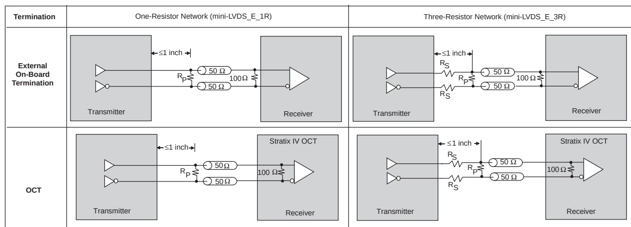
Figure 6-35. Mini-LVDS I/O Standard Termination (1)
