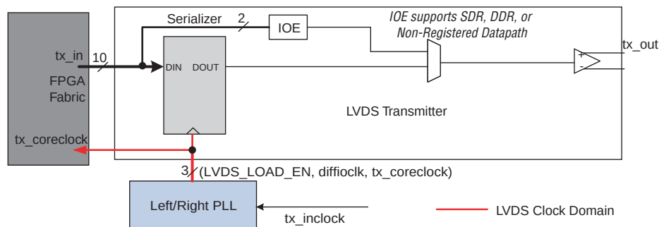
Figure 8-5. Stratix IV Transmitter (1), (2)
