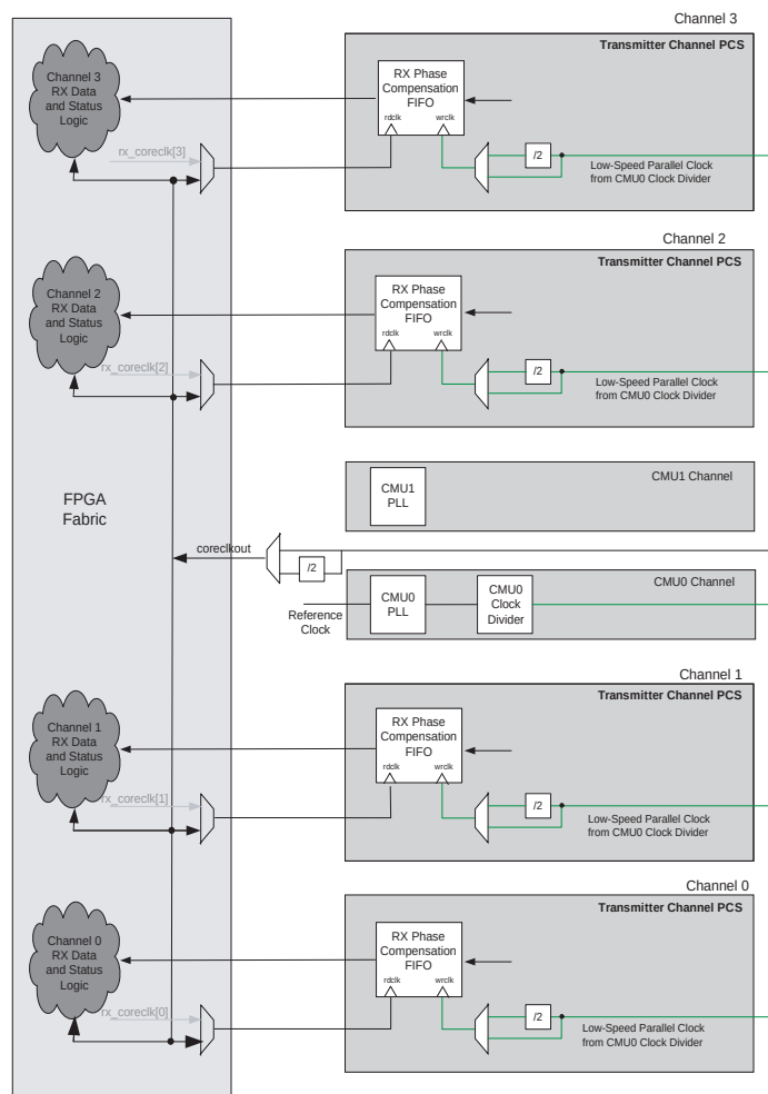
Figure 2–35. FPGA Fabric-Receiver Interface Clocking in a ×4 Bonded Channel Configuration (1)
