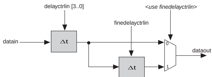
Figure 7-33. Delay Chain
