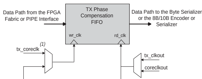
Figure 1-14. TX Phase Compensation FIFO
