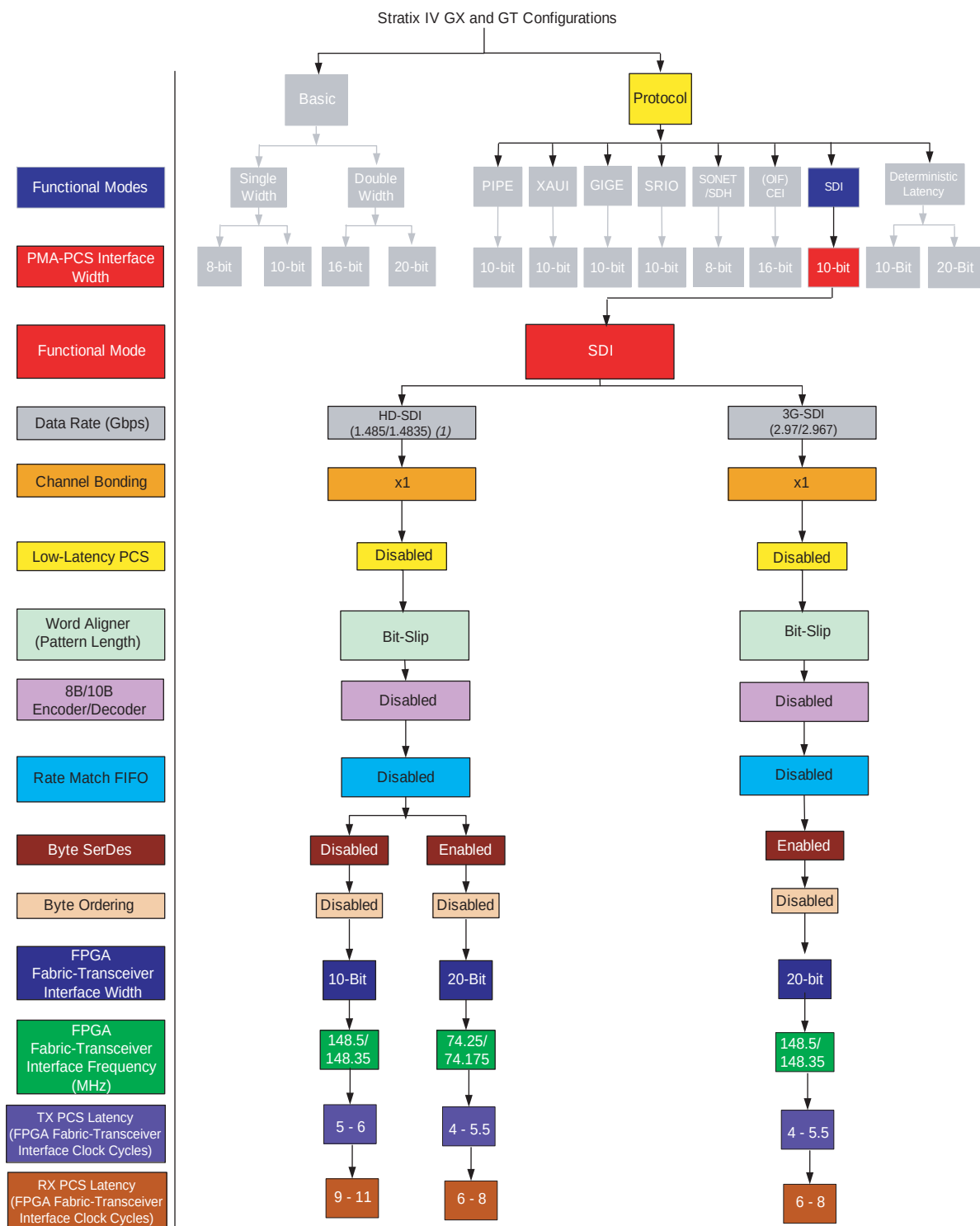
Figure 1-145. SDI Mode
