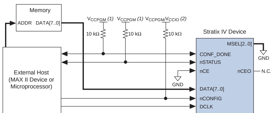
Figure 10-1. Single Device FPP Configuration Using an External Host
