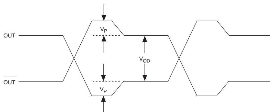
Figure 8-9. Programmable Pre-Emphasis (1)
