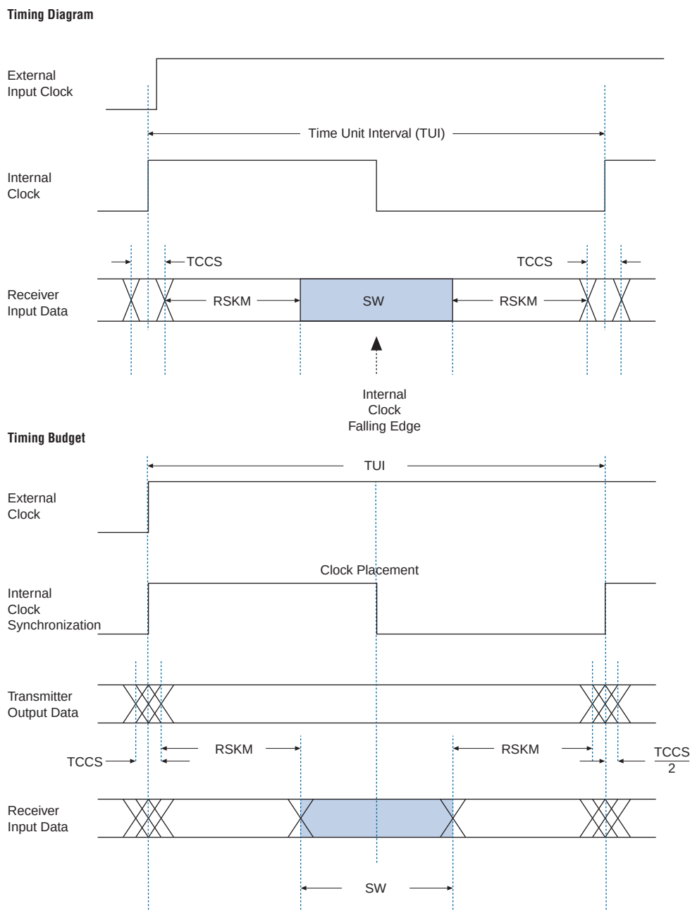
Figure 8-27. Differential High-Speed Timing Diagram and Timing Budget for Non-DPA Mode
