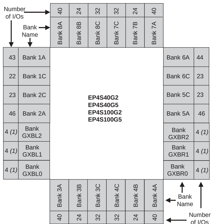
Figure 6-16. Number of I/Os in Each Bank in EP4S40G2, EP4S40G5, EP4S100G2, and EP4S100G5 Devices in the 1517-Pin FineLine BGA Package (1)
