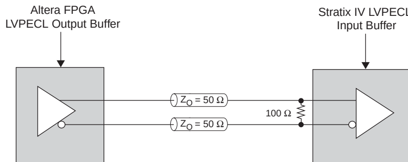
Figure 6-33. LVPECL DC-Coupled Termination (1)
