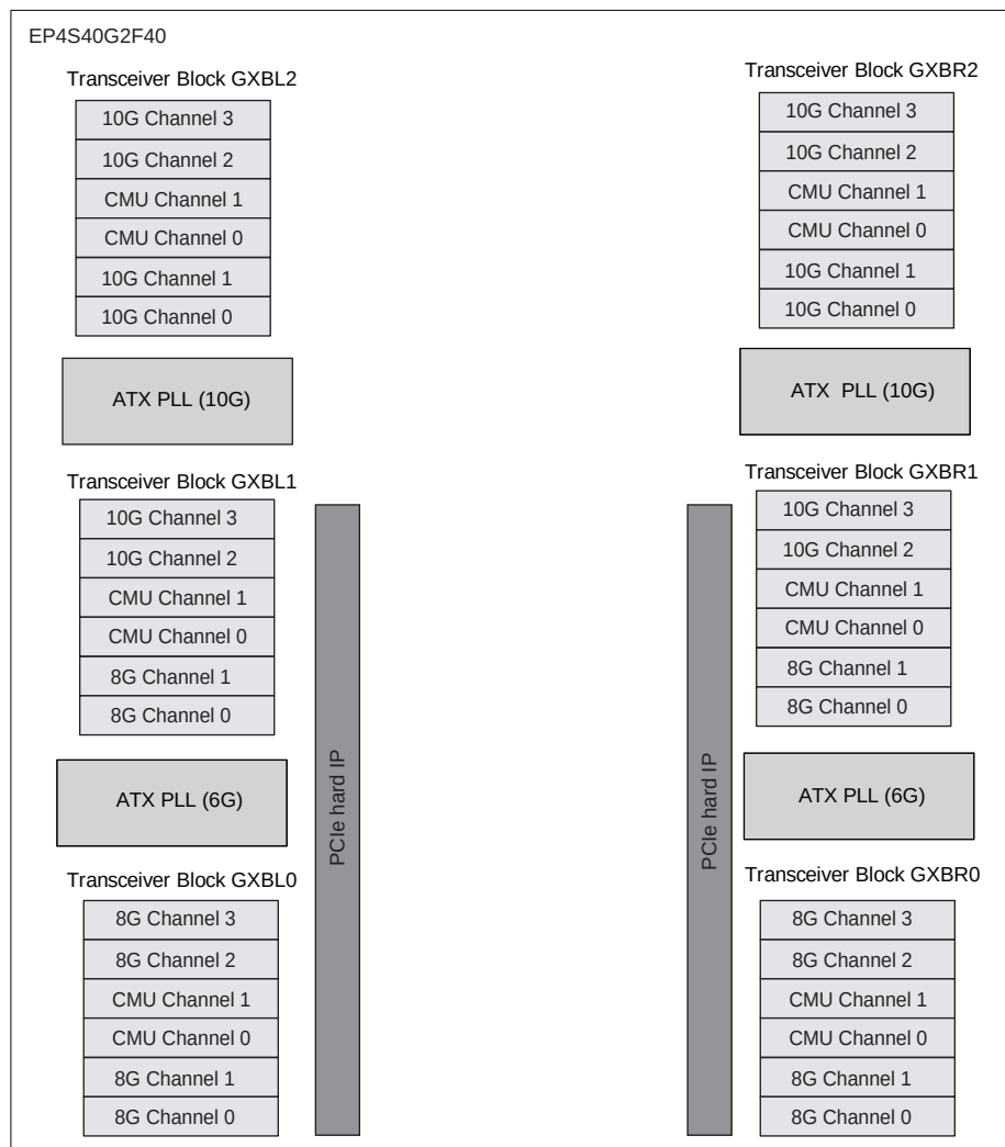
Figure 1–5. Transceiver Channel, PLL, and PCIe Hard IP Block Locations in EP4S40G2F40 Stratix IV GT Devices (1), (2)
