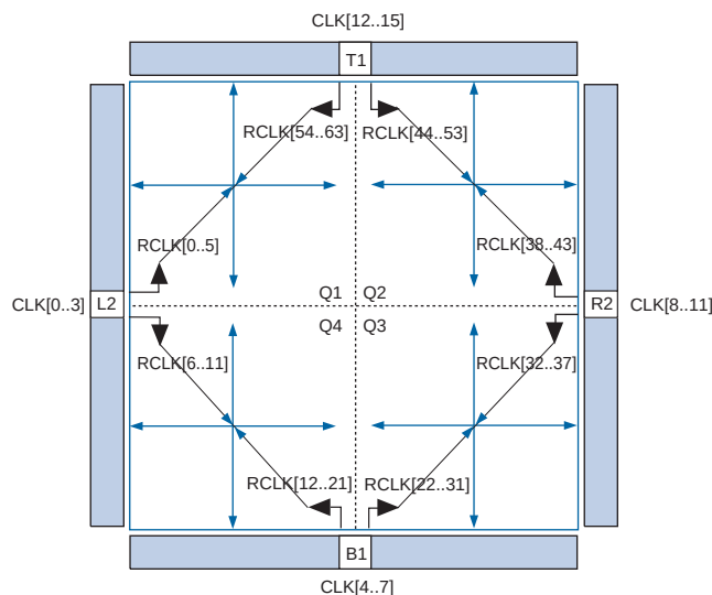
Figure 5-2. RCLK Networks (EP4SE230, EP4SGX70, and EP4SGX110 Devices) (1)
