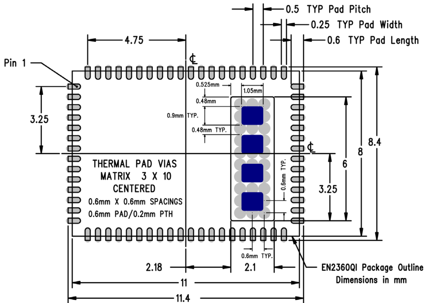
Figure 15: EN2360QI PCB Footprint (Top View)
