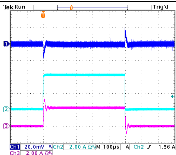
Load Transient Response: AVIN = 3.3V , VDDQ = 1.5V , VOUT = VDDQ \cdot 0.5 , Ch.1: V_{OUT} , Ch.2: I_{LOAD} 0 \leftrightarrow \sim 4A , Ch.3: I_{VDDQ} C_{IN} = 2 \times 47\mu F (0805), C_{OUT} = 4 \times 100\mu F (1206)
