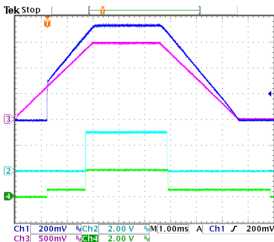
Power Up/Down into a \sim 94m\Omega Load: AVIN = 3.3V , VDDQ = 1.5V , VOUT = VDDQ \cdot 0.5 , Ch.1: V_{OUT} , Ch.2: VDDQOK , Ch.3: VDDQ , Ch. 4: POK C_{IN} = 2 \times 47\mu F (0805), C_{OUT} = 4 \times 100\mu F (1206)
