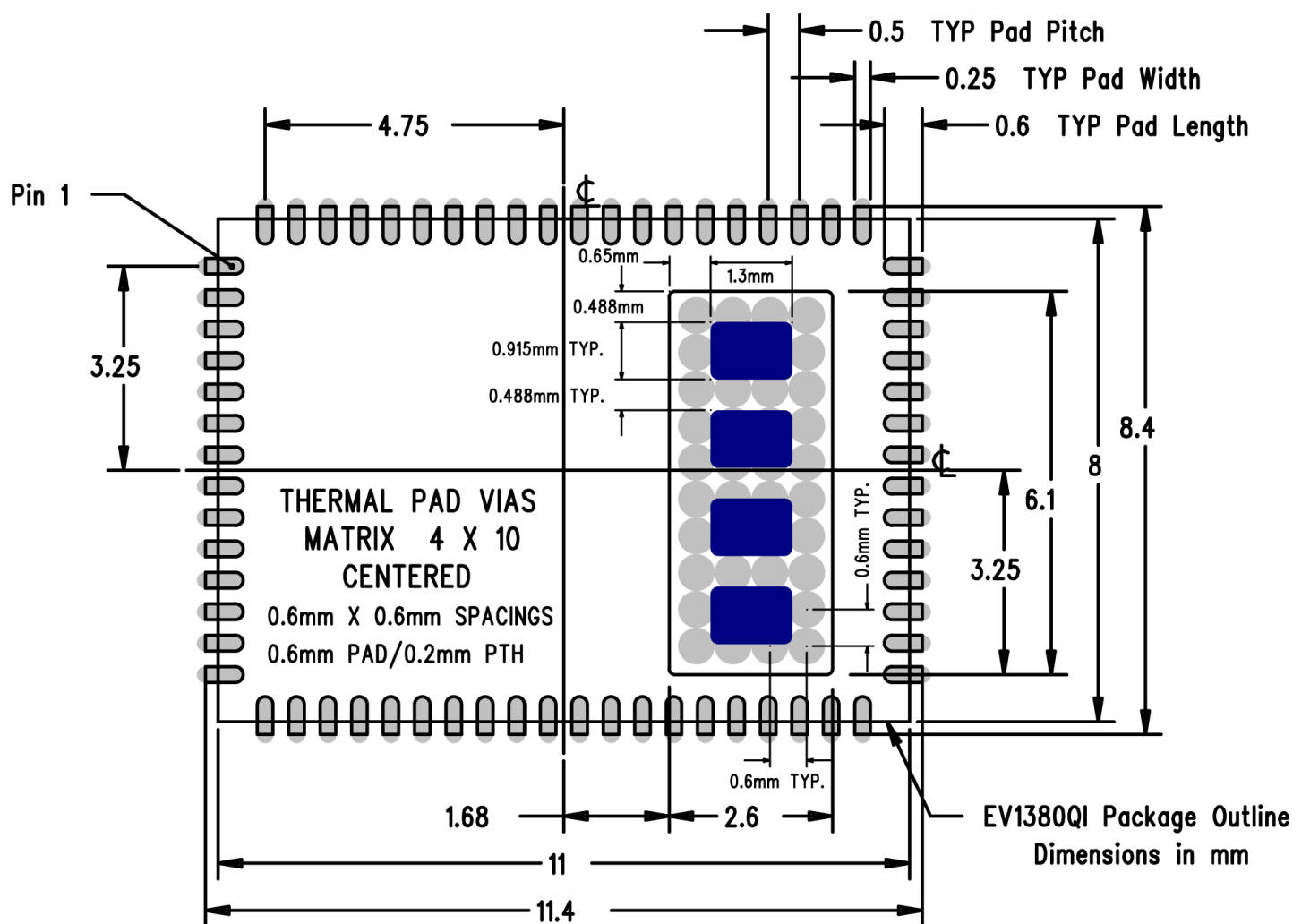
Figure 11: EV1380QI PCB Footprint (Top View)
