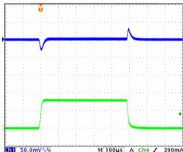
Transient, V_{IN} = 3.3V , V_{OUT} = 1.2V , Load = 0-800mA.
