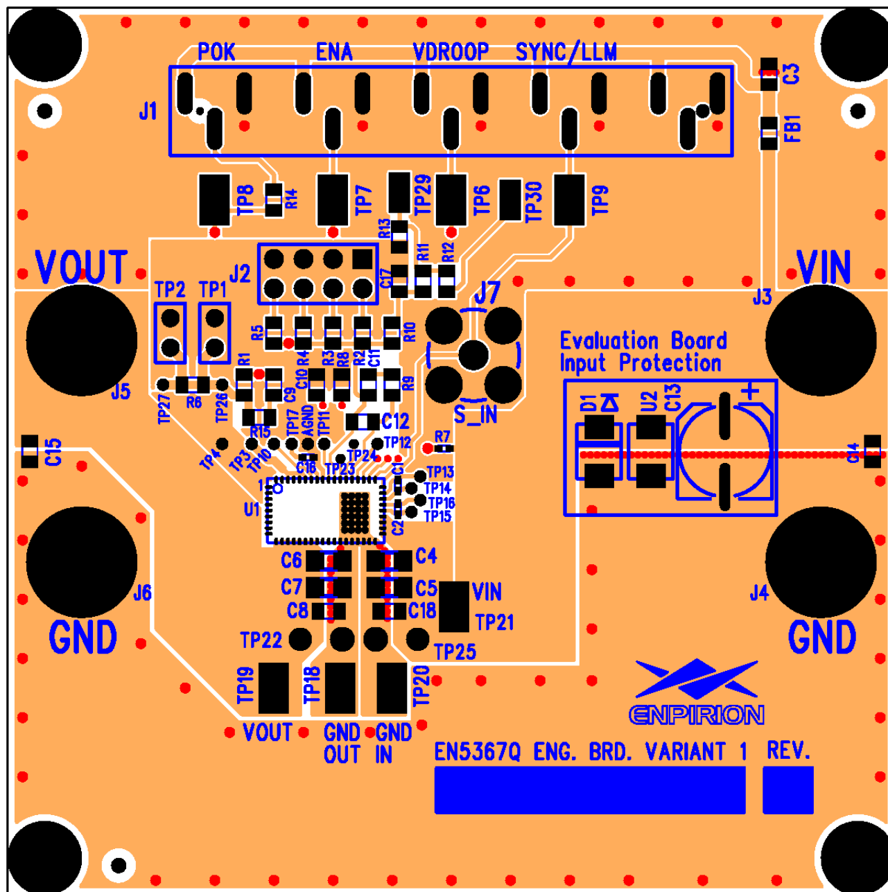
Figure 4: Evaluation Board Layout Top and Assembly Layers
