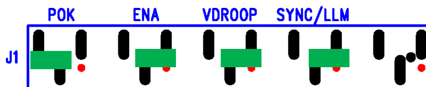
Figure 1: Shows POK, Enable, VDROOP and SYNC/LLM Jumpers. POK PWR jumper as shown connects the pull-up resistor to VIN. Enable jumper shown is in DISABLE position. SYNC/LLM jumper as shown ties this pin Low. VDROOP jumper as shown is low, and should stay grounded.
