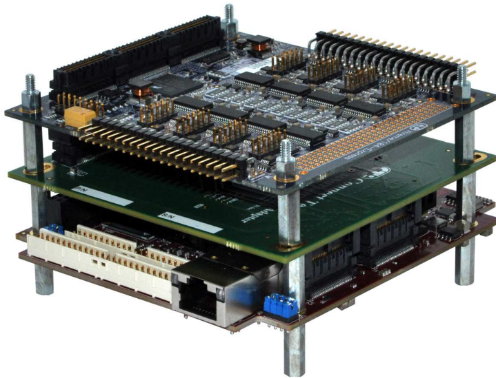
SUMIT-104 stack configuration
