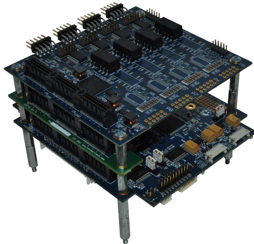
PCIe/104 Bus Extender in a Stack Configuration
