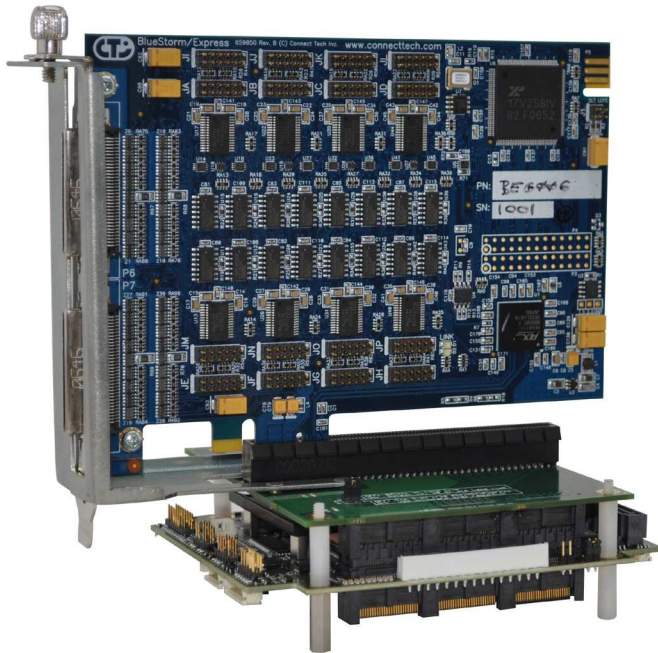
ADG017 with PCIe/104 SBC card and PCI Express card installed
