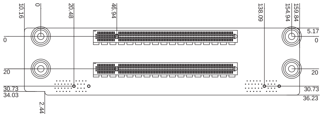
Mechanical Diagram
