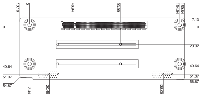
Mechanical Diagram
