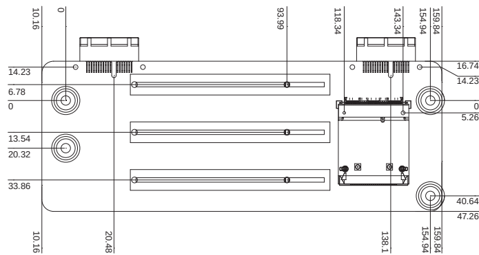
Mec h a n i c a l D i a g r a m
