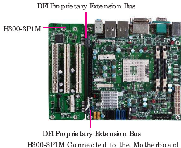
H300-3P1M Connected to the Mo the r b o a r d
