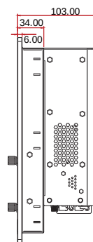
Right View
