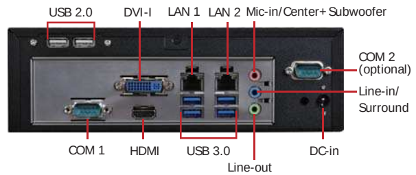
Rear View
