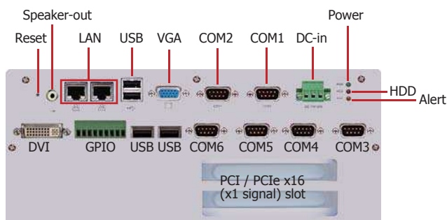
EC220/ 221-BTA881 Rear View
