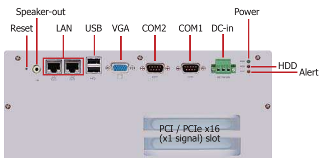
EC220/ 221-BT6060 Rear View
