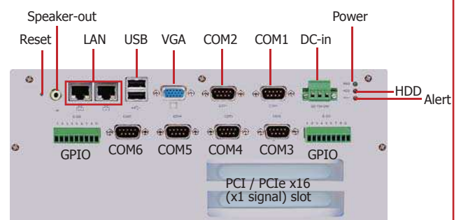
EC220/ 221-BTAG60 Rear View
