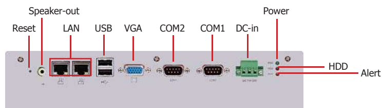
EC200-BT6060 Rear View
