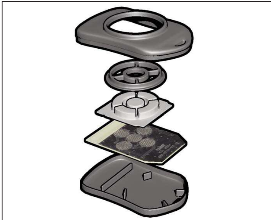
Figure 5: OTX-***-HH-KF#-MS Assembly
