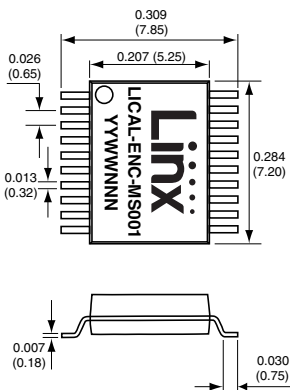
Figure 1: Package Dimensions
