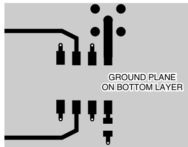
Figure 17: Suggested PCB Layout
