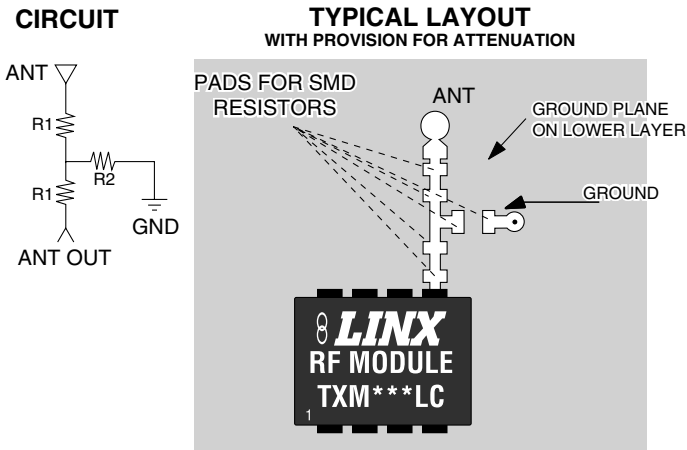
Figure 14: A T-Pad Attenuator Layout Example
