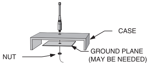
Figure 27: Remote Ground Plane
