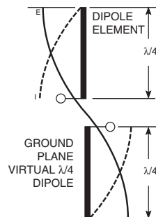
Figure 26: Dipole Antenna
