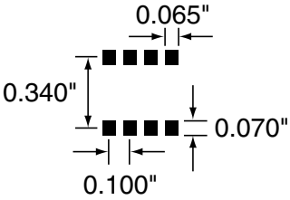
Figure 20: Recommended PCB Layout
