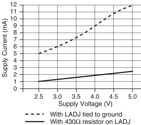
Figure 6: Current vs. Supply Voltage
