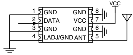
Figure 5: Test / Basic Application Circuit
