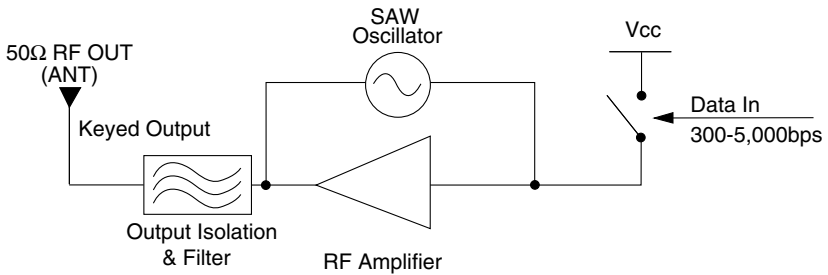
Figure 13: LC Series Transmitter Block Diagram
