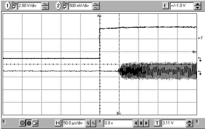
Figure 8: Typical Oscillator Turn-On Time
