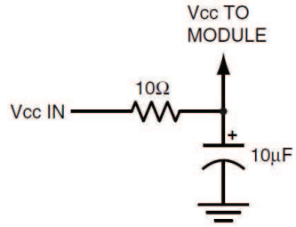
Figure 15: Supply Filter
