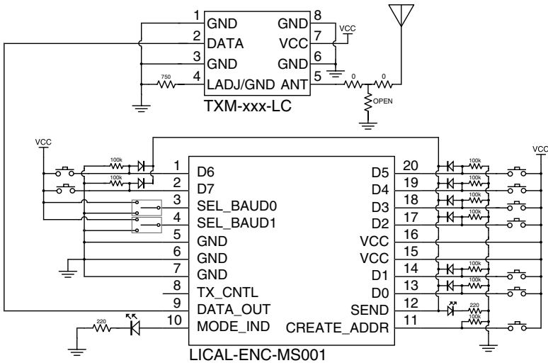
Figure 16: Typical Remote Control Example
