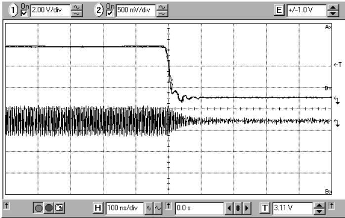
Figure 9: Oscillator Turn-Off Time
