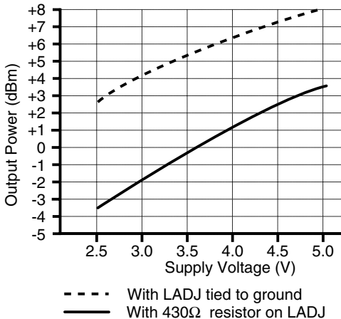
Figure 7: Output Power vs. Supply Voltage
