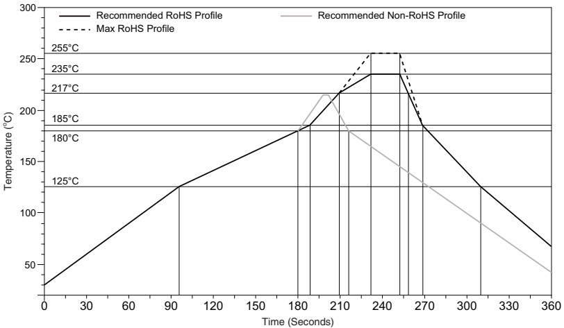
Figure 23: Maximum Reflow Profile
