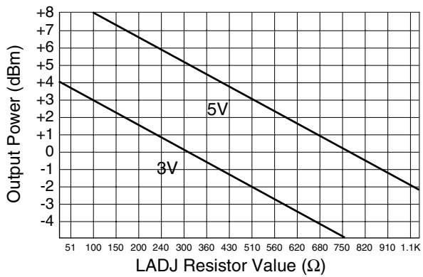
Figure 10: Output Power vs. LADJ Resistor
