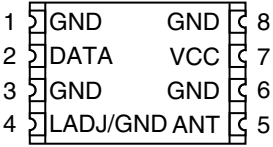
Figure 11: LC Series Transmitter Pinout (Top View)
