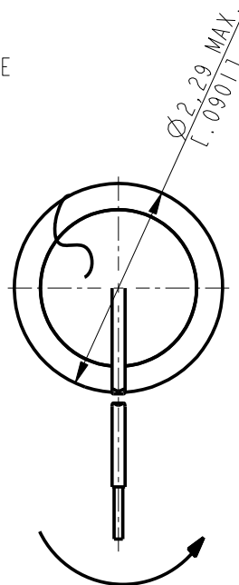
COIL WIRE WINDING DIRECTION
