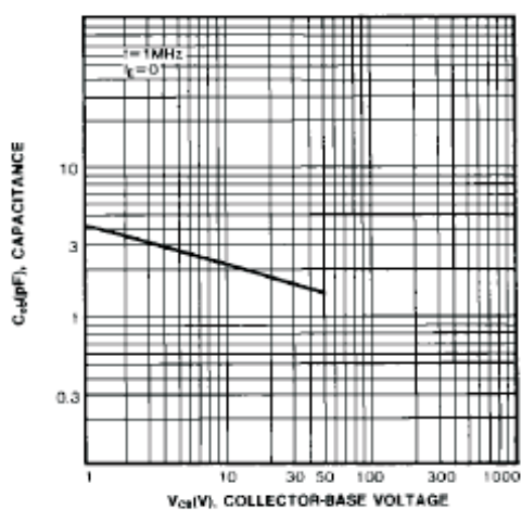
Fig.6 Output Capacitance
