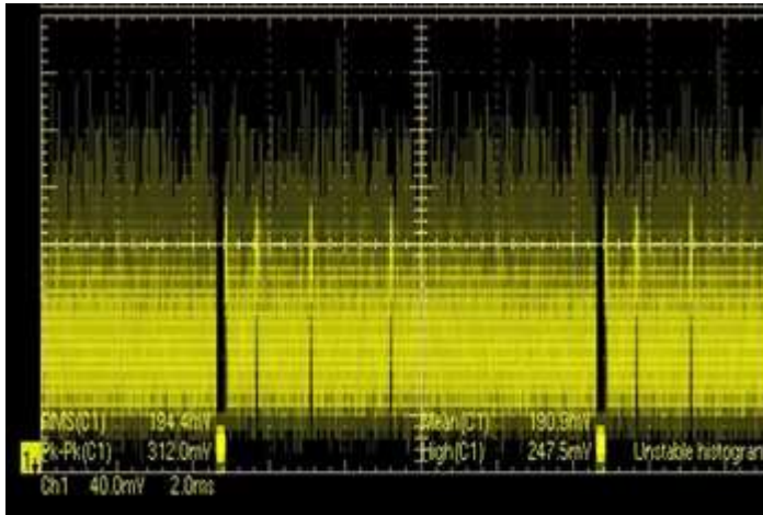
Figure 11 RF Envelope
