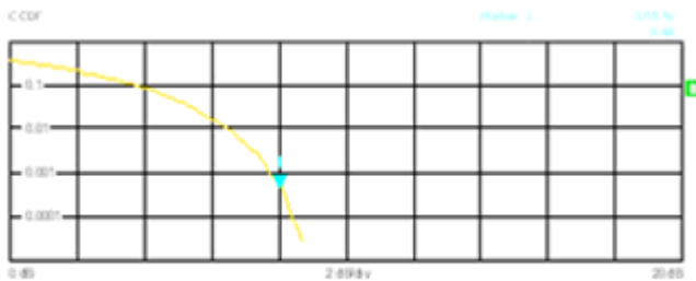
Figure 13 CCDF
