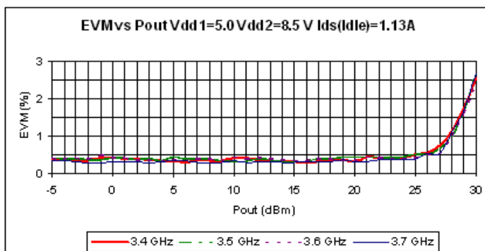
Figure 15 EVM vs Pout
