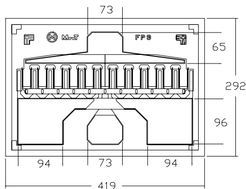
Chip Dimensions: 419 x 292 microns Chip Thickness: 100 microns
