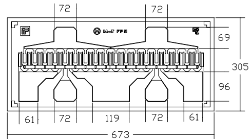
Chip Dimensions: 673 x 305 microns Chip Thickness: 100 microns
