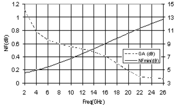
NF & Associated Gain vs. Freq Vds = 2.5V, Ids = 50mA
