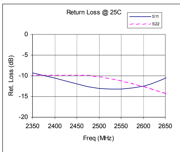
Figure 3B: Ret. Loss, 2400-2600 MHz
