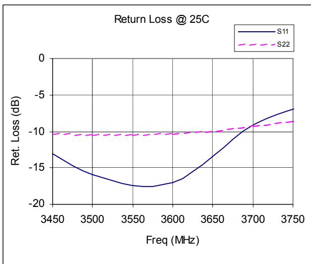
Figure 4B: Ret. Loss, 3500-3700 MHz
