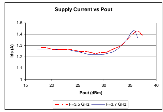
Figure 3 Supply Current
