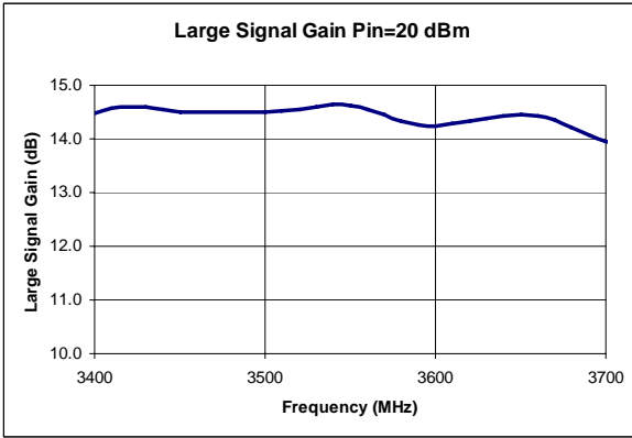
Figure 4 Gain Response
