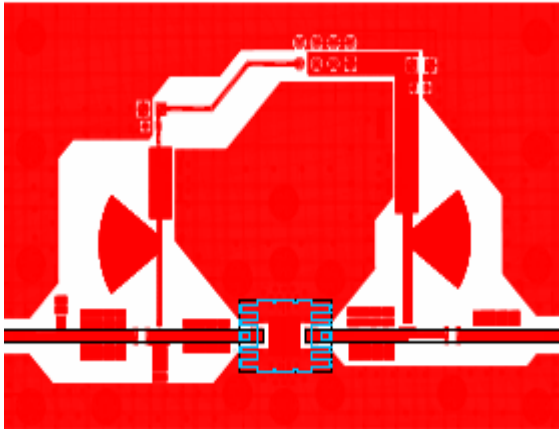
Figure 1 Evaluation board
