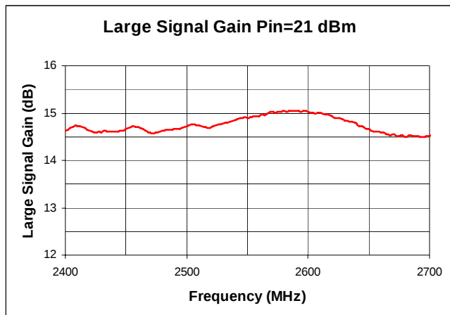
Figure 4 Gain Response
