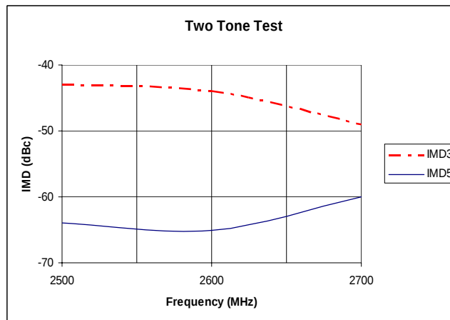
Figure 5 OIP3
