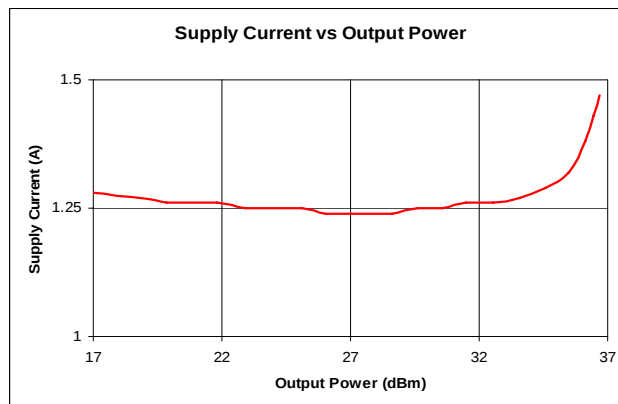
Figure 3 Supply Current
