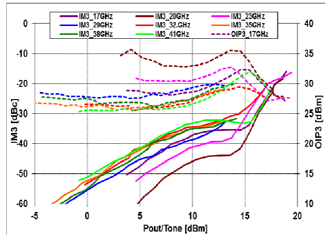
IM3 level [dBc] vs. Input power [dBm/ton]
