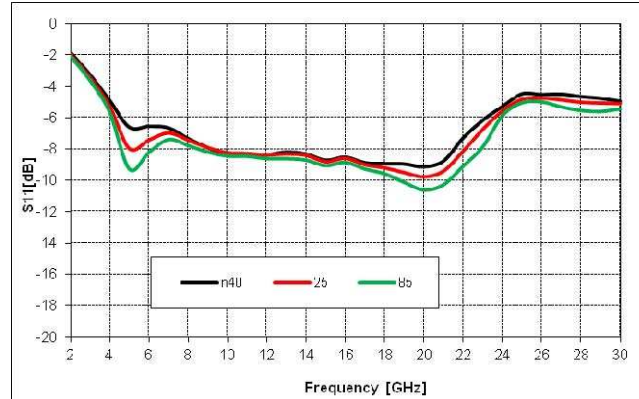
S11(dB) over temperature
