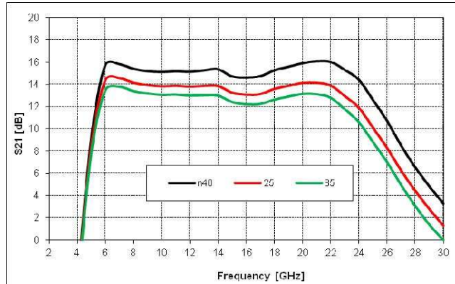
S21(dB) over temperature
