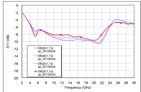
S11(dB) over Voltage
