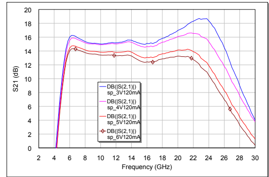
S21(dB) over voltage
