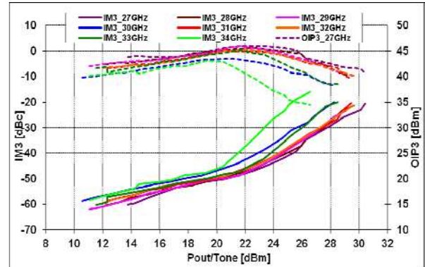
@ V_{ds}=4V , I_{dsq}=3.8A
