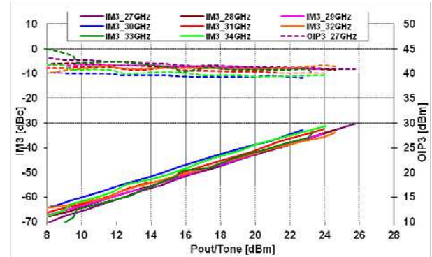
@Vds=5V, Idsq=2.4A
