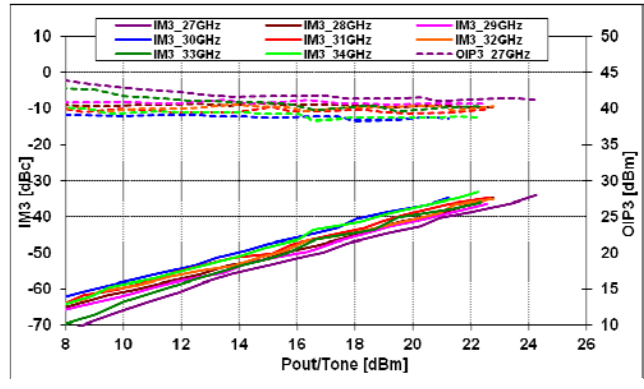
@Vds=6V, Idsq=2.4A
