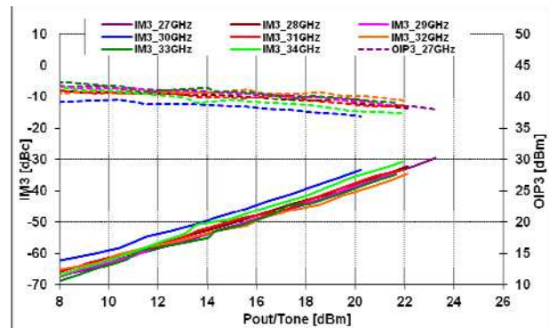
@Vds=5V, Idsq=1.5A
