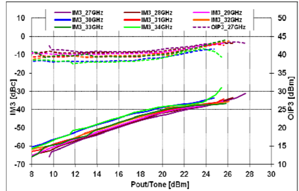
@Vds=5V, Idsq=3.3A
