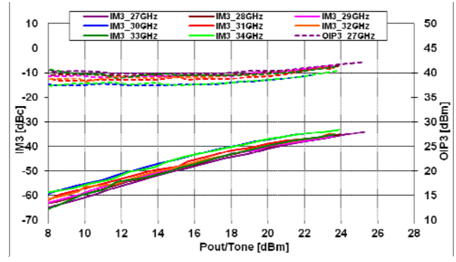
@Vds=6V, Idsq=3.3A
