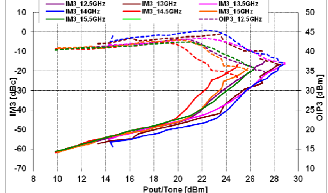
@ V_{ds}=4V , I_{dsq}=2000mA
