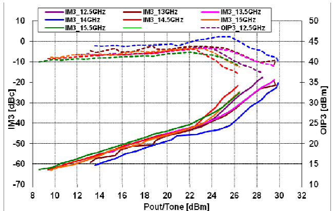
@ V_{ds}=5V , I_{dsq}=2000mA
