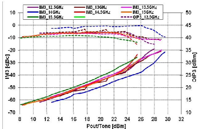
@ V_{ds}=5V , I_{dsq}=1400mA
