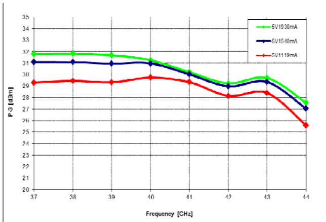
P-3 vs. Frequency
