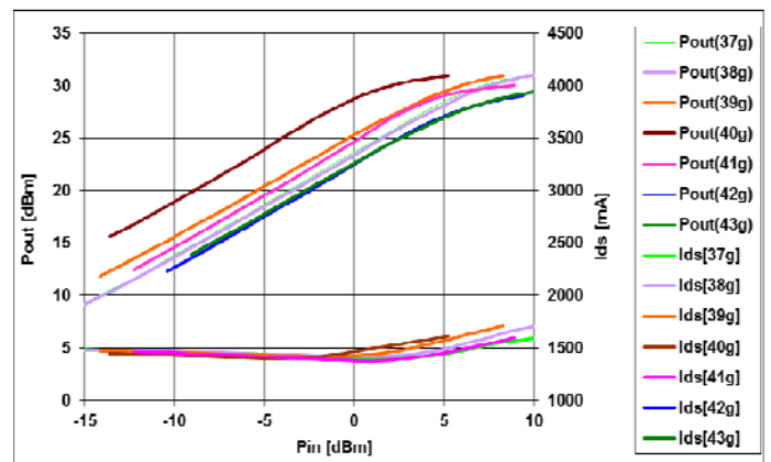
Po(dBm), Gain(dB), and Ids(mA) vs. Pin(dBm)
