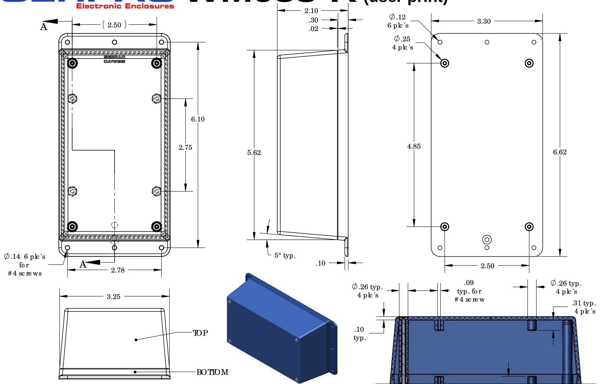
SECTION A-A SCALE 1 : 1.73
